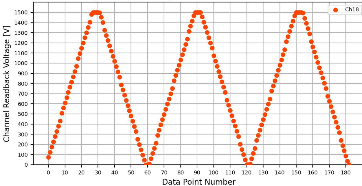
Voltage Ramp Test (Python) Bd #064, Slot #12, Ch #18
