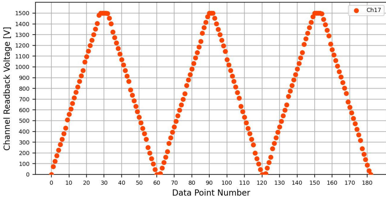
Voltage Ramp Test (Python) Bd #064, Slot #12, Ch #17
