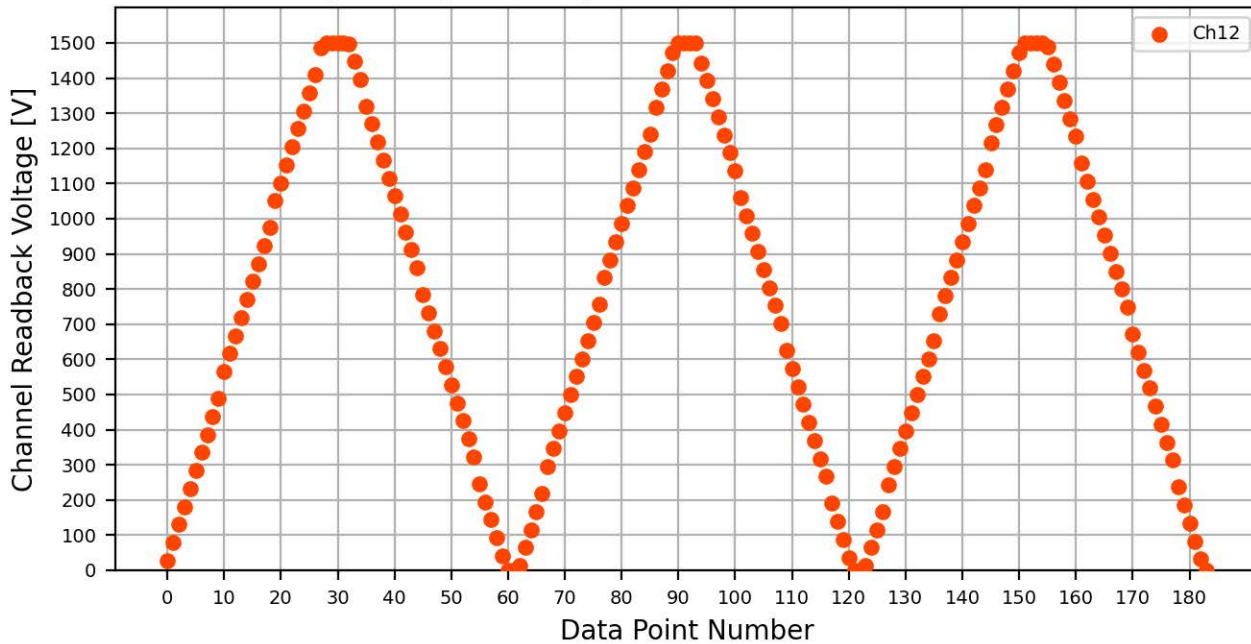
Voltage Ramp Test (Python) Bd #064, Slot #12, Ch #12
