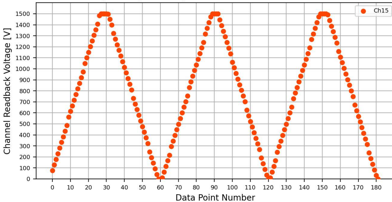
Voltage Ramp Test (Python) Bd #064, Slot #12, Ch #15
