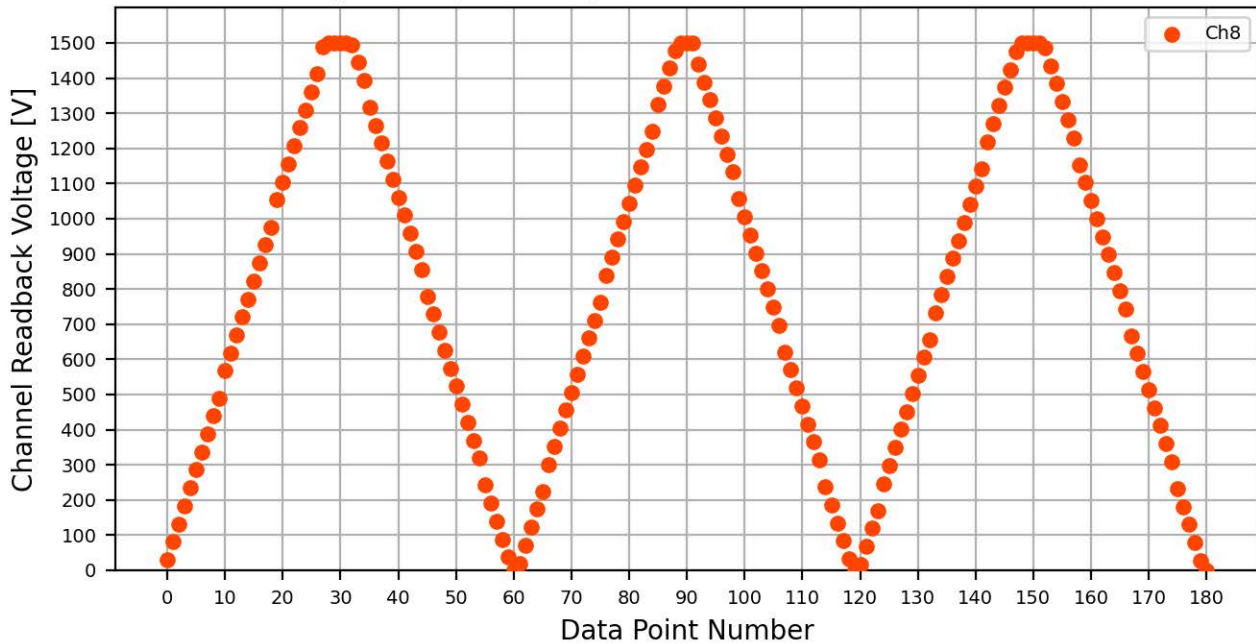
Voltage Ramp Test (Python) Bd #064, Slot #12, Ch #8
