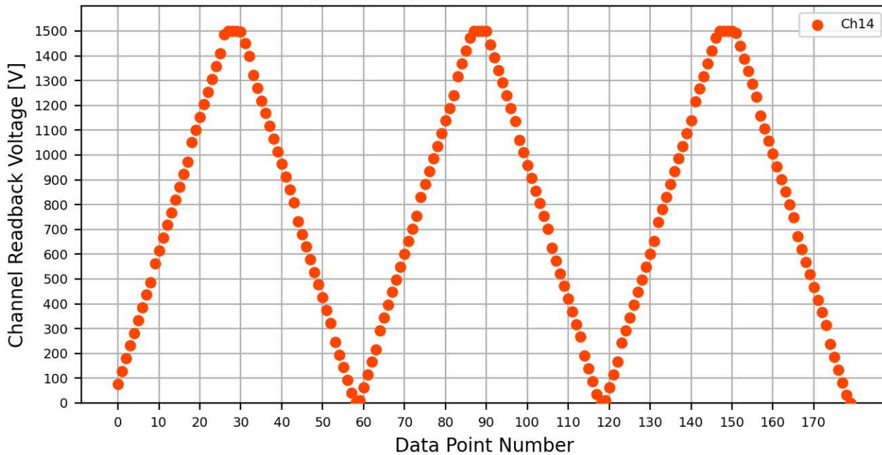
Voltage Ramp Test (Python) Bd #064, Slot #12, Ch #14
