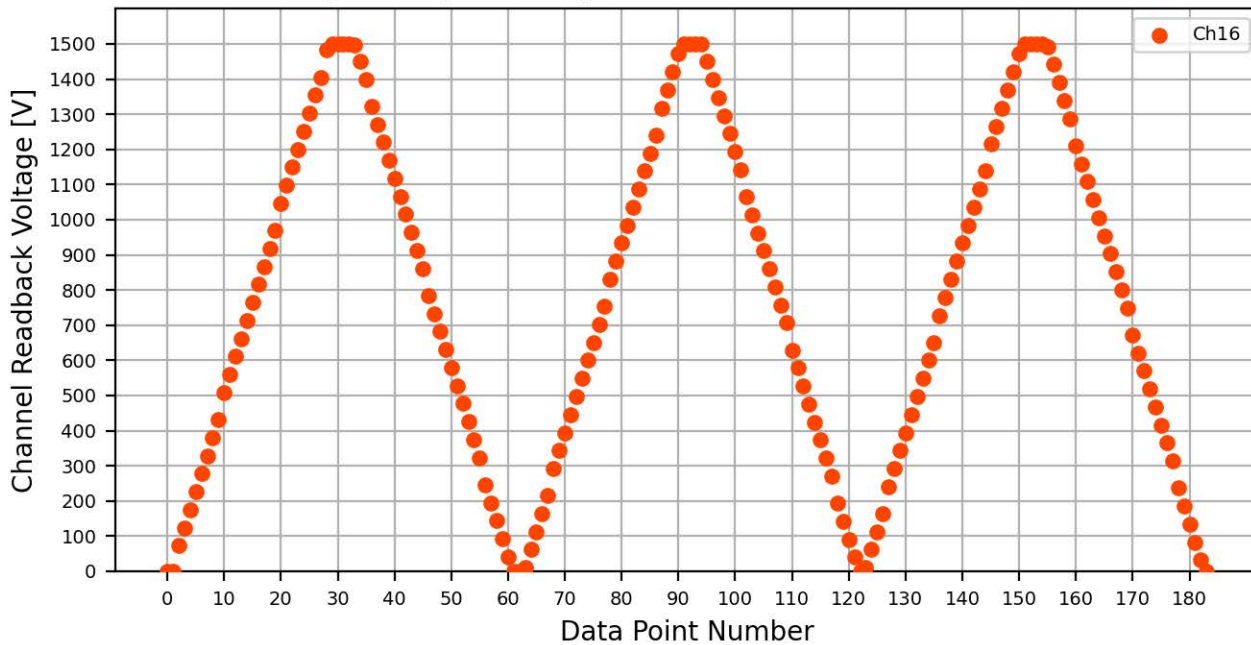
Voltage Ramp Test (Python) Bd #064, Slot #12, Ch #16
