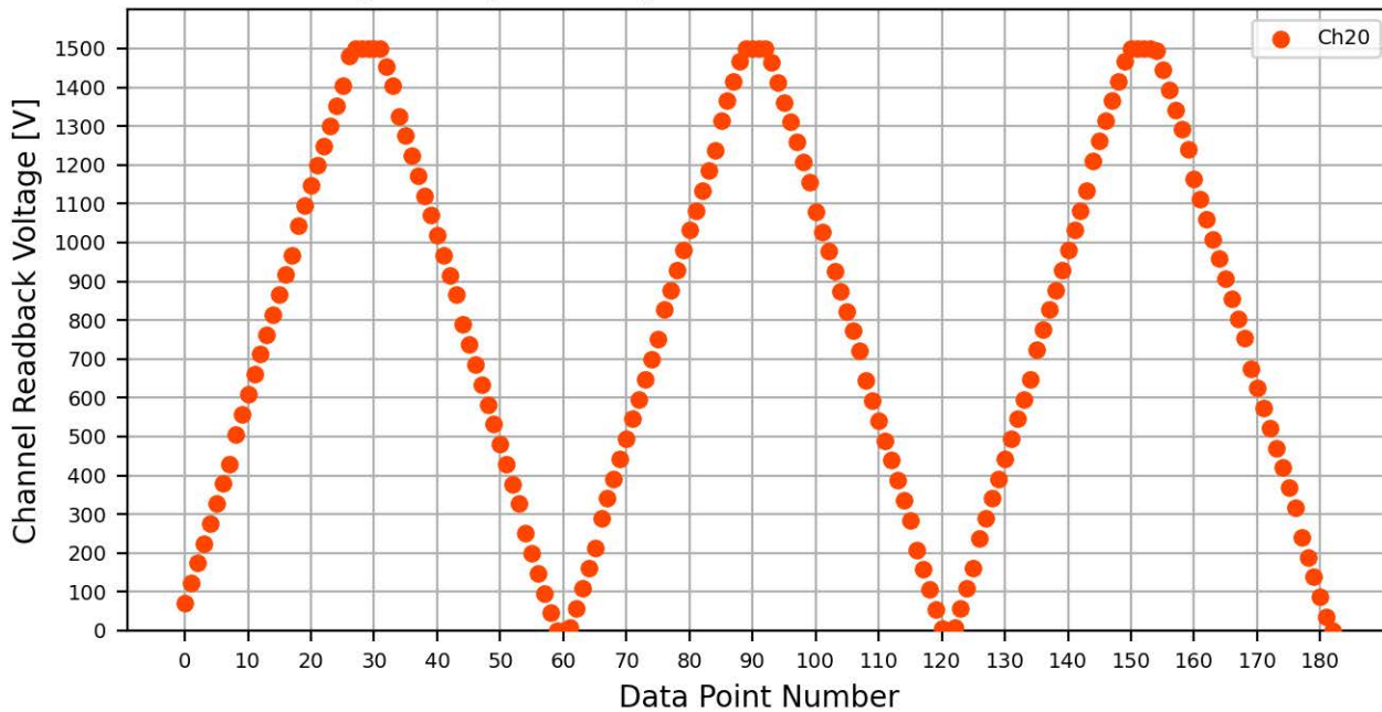
Voltage Ramp Test (Python) Bd #064, Slot #12, Ch #20
