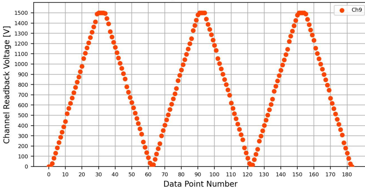
Voltage Ramp Test (Python) Bd #064, Slot #12, Ch #9
