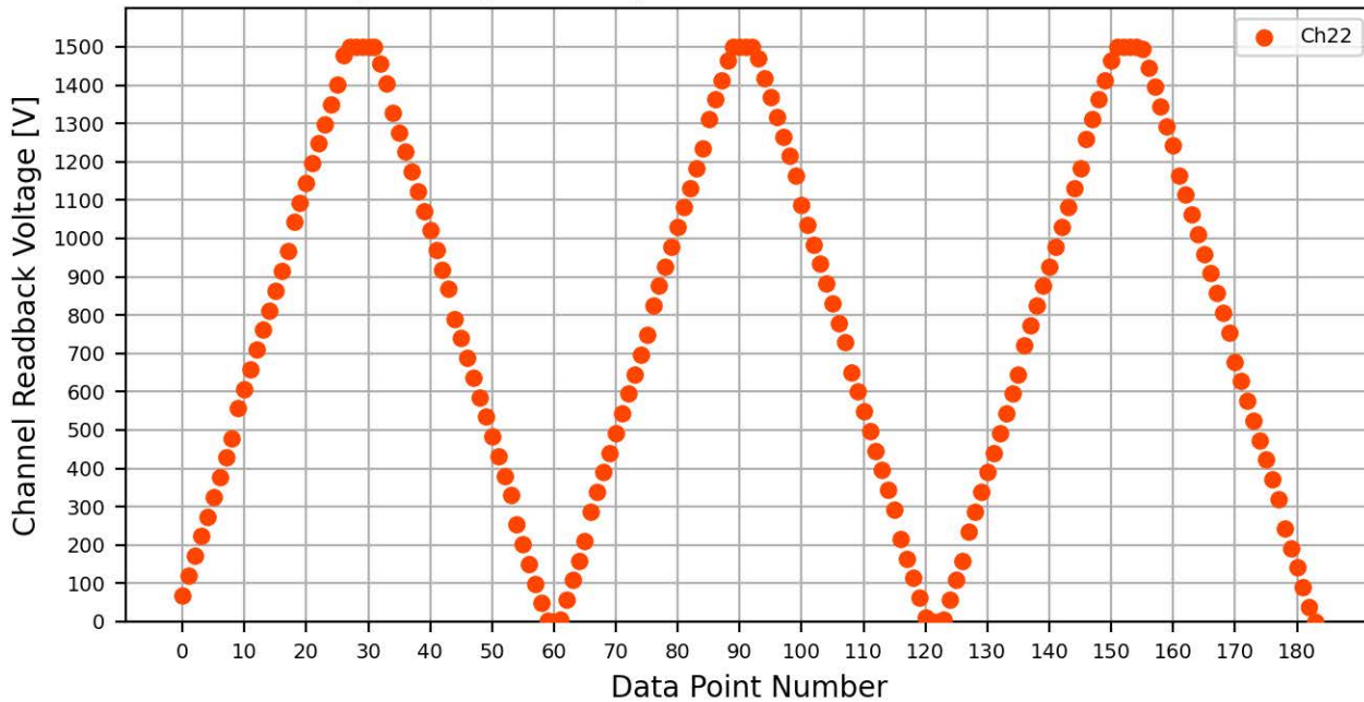
Voltage Ramp Test (Python) Bd #064, Slot #12, Ch #22
