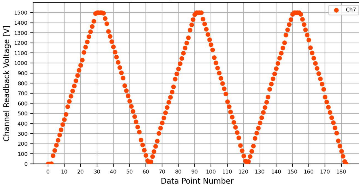
Voltage Ramp Test (Python) Bd #064, Slot #12, Ch #7
