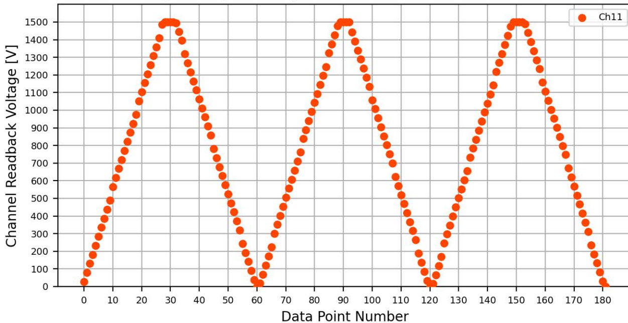
Voltage Ramp Test (Python) Bd #064, Slot #12, Ch #11
