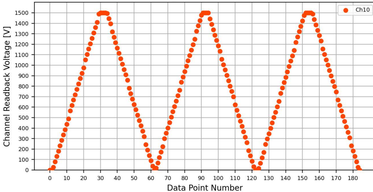
Voltage Ramp Test (Python) Bd #064, Slot #12, Ch #10
