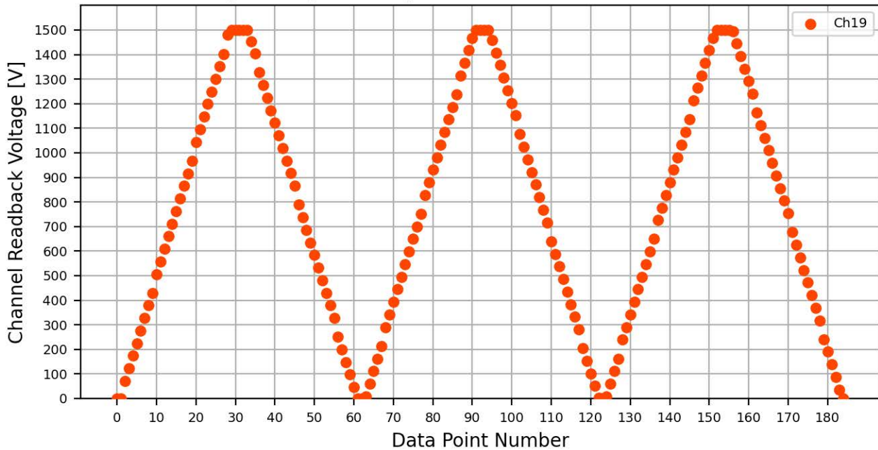
Voltage Ramp Test (Python) Bd #064, Slot #12, Ch #19
